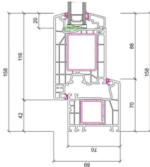
Double Glazed OUTSWING
