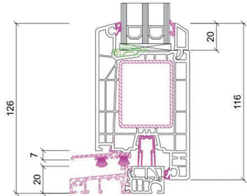
Triple Glazed INSWING
