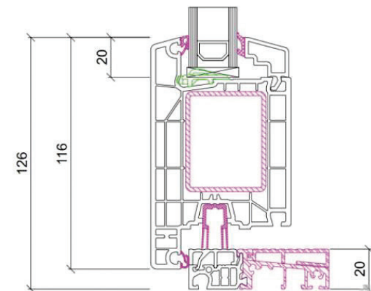
Double Glazed OUTSWING
