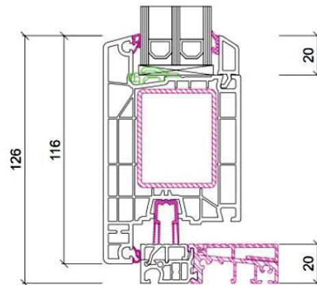
Triple Glazed OUTSWING
