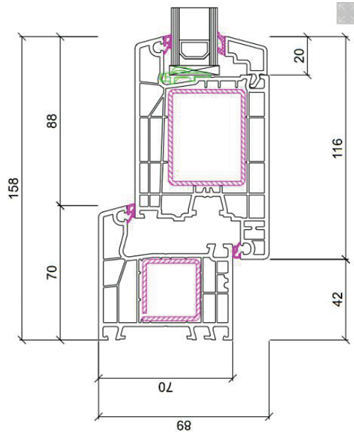
Double Glazed INSWING
